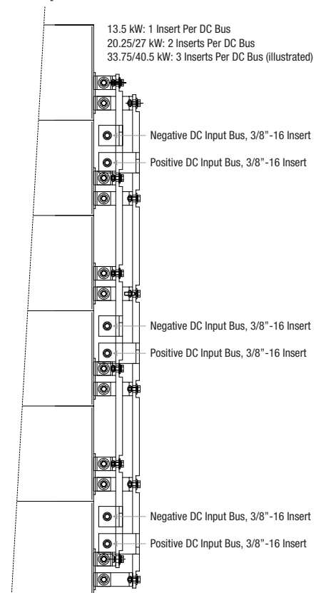
DC Input Bus 13.5 kW to 40.5 kW Models
