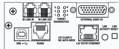
Rear communication interfaces with LXI TCP/IP Ethernet (+LXI) option.
