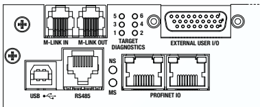
Rear communication interfaces with PROFINET (+PROF) option.
