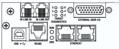
Rear communication interfaces with EtherCAT (+ECAT) option.
