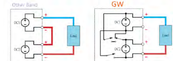
Output in Series Connections
