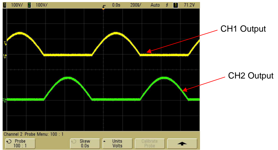
Figure 2-6, Amplified Unipolar Sine Waveform
